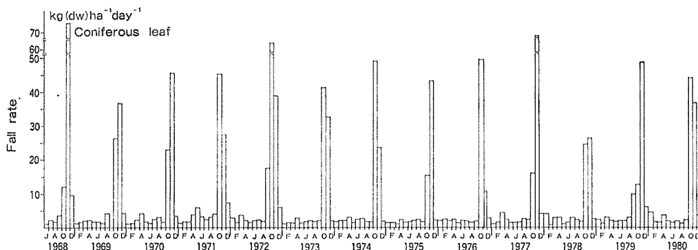
Fig. 3. Seasonal fluctuations in the fall rates of leaf litter in fir-hemlock mixed stand
