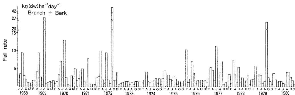
Fig. 4. Seasonal fluctuations in the fall rates of branch litter (including bark) in fir-hemlock mixed stand
