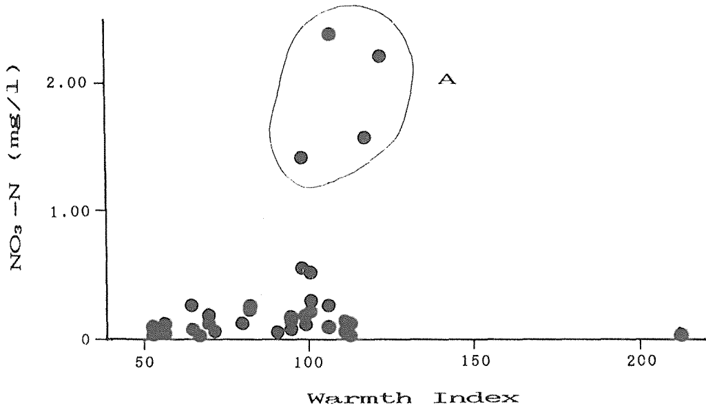
図4 硝酸態窒素 (NO 3 -N) 濃度と暖かさの指数の関係 A : Nod21, No. 25, No. 26, No. 32 (岡山, 香川) Fig.4 Relationship between concentration of nitrate-nitrogen and Warmth Index.
