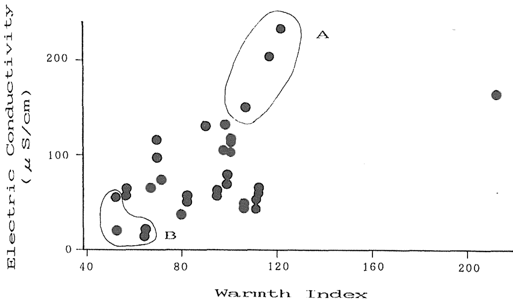
図2 電気伝導度と暖かさの指数の関係 A : No. 21, No. 26, No. 32 (岡山, 香川) B : No. 13, No. 14, No. 33, No. 34 (岐阜, 長野) Fig. 2 Relationship between Electric Conductivity and Warmth Index
