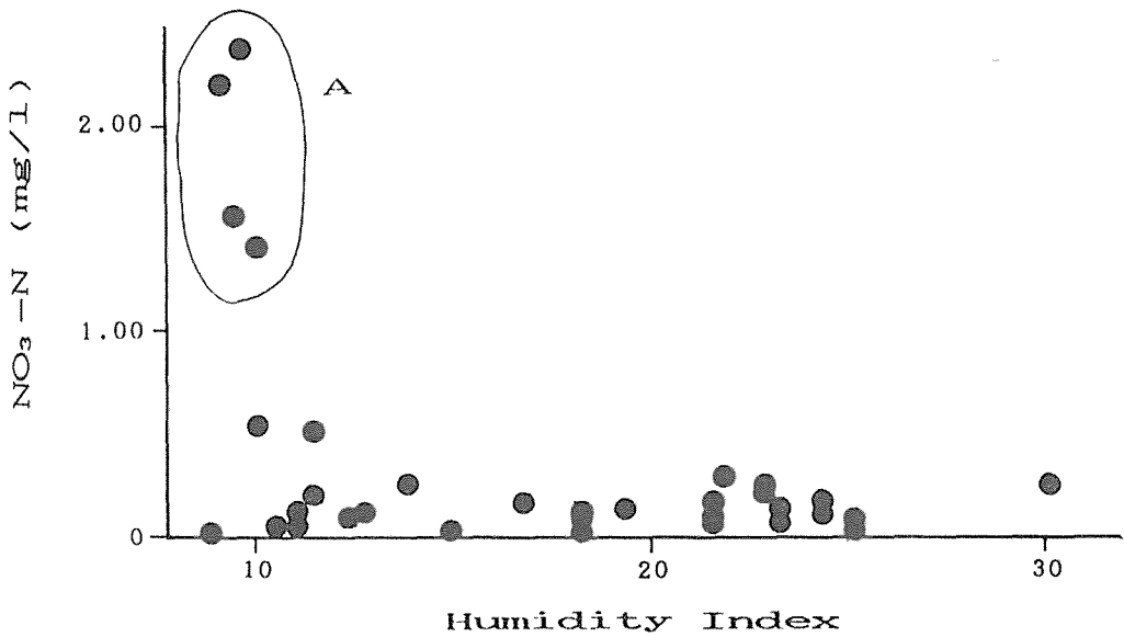
図5 硝酸態窒素 (NO 3 -N) 濃度と乾湿指数の関係 A : No. 21, No. 25, No. 26, No. 32 (岡山, 香川) Fig.5 Relationship between nitrate-nitrogen and Humidity Index.
