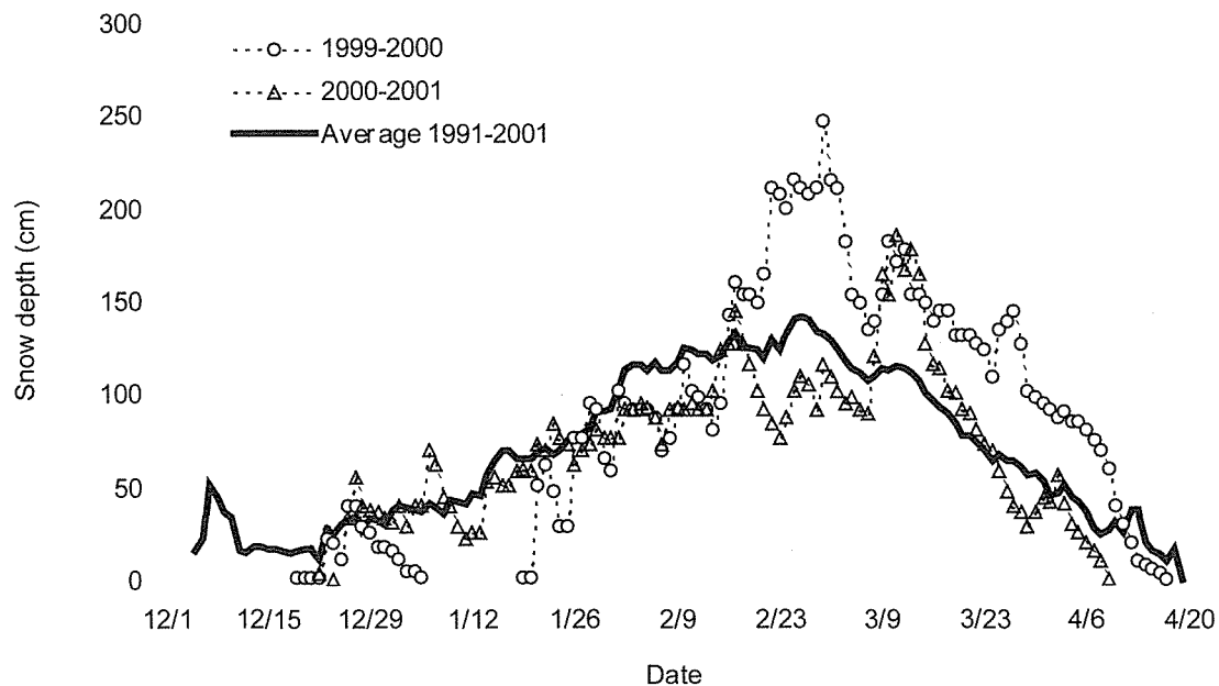
Figure 2. Snow depth at the meteorological station of Ashiu Research Forest during two winter periods (1999-2000 and 2000-2001) and the average snow depth in recent 10 years (1991 to 2001).
