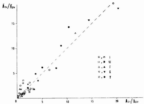
Fig. 9. Theoretical and observed amplitude-ratios of P - and SV -waves at the respective stations in case of conical type. (abscissa: theoretical ratio, ordinate: observed ratio) Empty symbols denote the initial amplitude-ratios, and filled symbols indicate the maximum amplitude-ratios.
