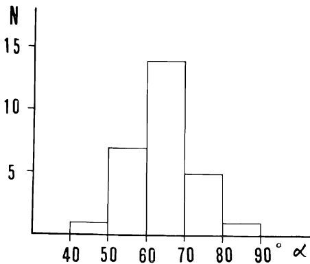
Fig. 12. Frequency distribution of \alpha .
