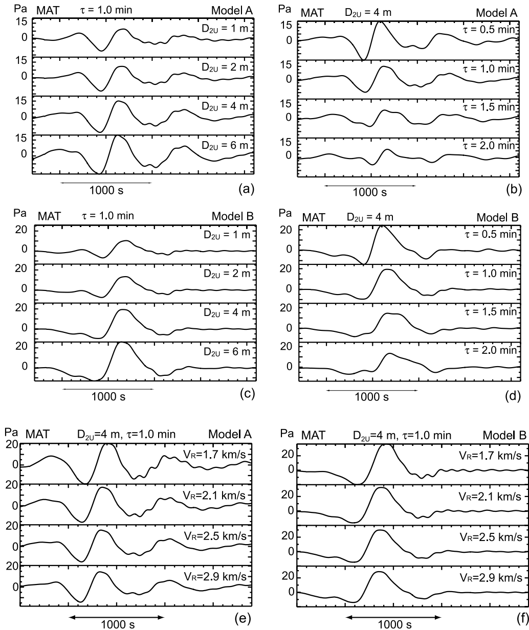
Figure 6. (a) and (c) Synthetic waveforms for MAT for four assumed displacements from D_{2U} with a fixed risetime of 1 min. (b) and (d) Synthetic waveforms for MAT for four assumed risetimes with a fixed displacement D_{2U} = 4 m and D_{2D} = -2 m. Displacements in other zones are fixed to be D_{jU} = 1 m and D_{jD} = -0.5 m. The source expanding velocity v is assumed to be 2.5 km/s. (e) and (f) Synthetic waveforms for MAT for four assumed horizontal expanding velocities ranging from 1.7 to 2.9 km/s, with a fixed displacement as in Figures 6b and 6d and a fixed risetime of 1 min.
