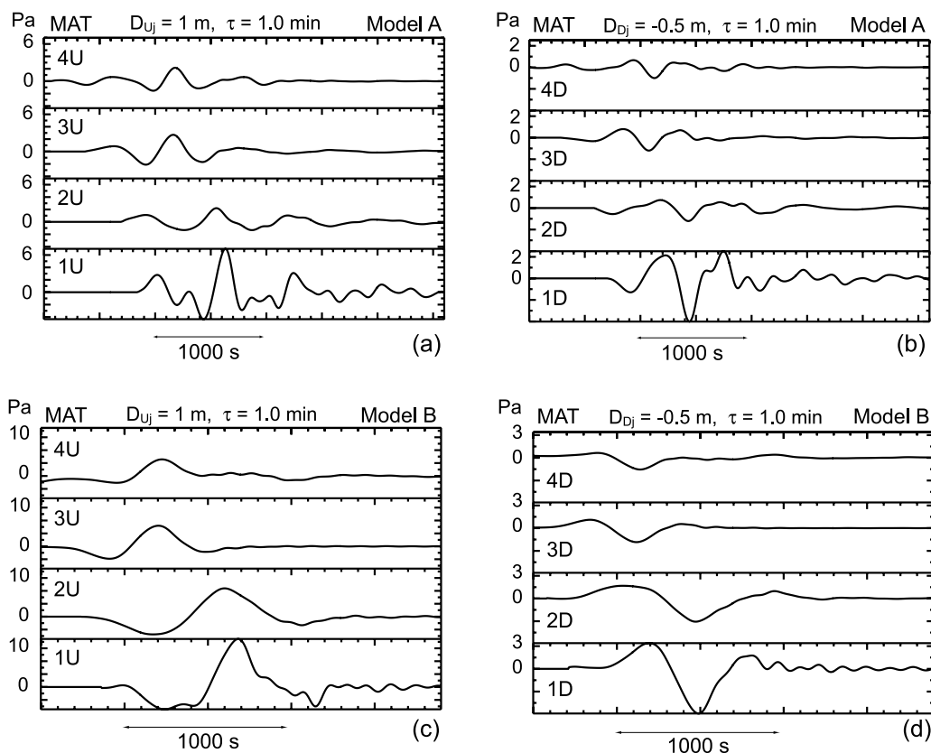
Figure 5. Synthetic waveforms for MAT coming from each of eight zones: (a) and (c) the uplifted zone and (b) and (d) the subsided zones. D_{jU} and D_{jD} are assumed displacements, and \tau is an assumed risetime. Models A and B correspond to two different atmospheric models (see text).
