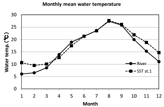
Fig.5 Monthly mean water temperature at Ise-Oohashi (river) and SST st.1 (ocean). Monthly mean data were calculated from 2001 to 2011.
