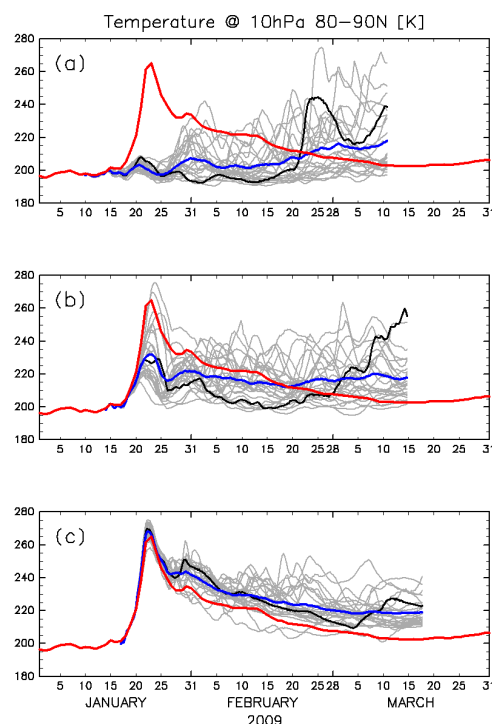
Fig. 3 Time evolution of 10-hPa north-polar temperature during a period from 1 January to 31 March 2009 (red line) and the ensemble forecasts (gray lines) starting from 10 (a), 14 (b), and 17 January (c). The blue line and the black line denote the ensemble mean and the control forecast, respectively.
