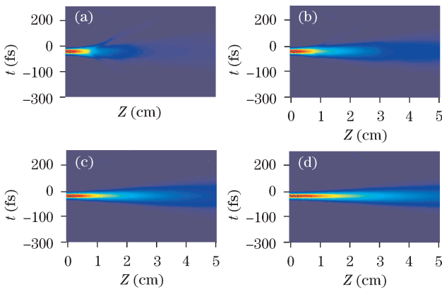
Fig. 3. Evolution of temporal profiles integrated over the beam radius within (a) 100\ \mu\text{m} , (b) 200\ \mu\text{m} , (c) 500\ \mu\text{m} , and (d) the whole space as a function of the propagation distance for a 10P_{cr} peak power incident pulse with a diameter of 100\ \mu\text{m} .
