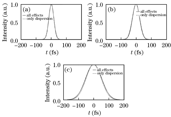
Fig. 2. Temporal profiles integrated over the beam radius of a 10P_{cr} peak power incident pulse with a diameter of 100\ \mu\text{m} with all the effects and only dispersion taken into account at z = (a) 1, (b) 2, and (c) 5 cm.
