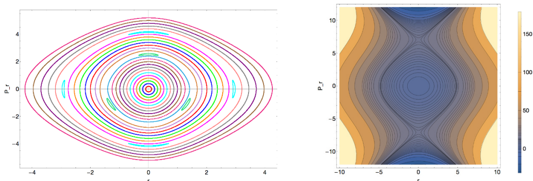
(a) Poincaré section with E = 10 . (b) Energy contours in the r-p_r phase space.
