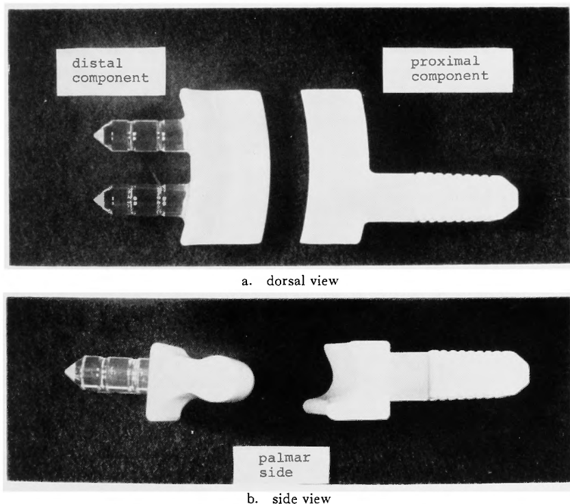
Fig. 1. Stable Cementless Wrist Prosthesis The proximal component consists of a quadrangular ceramic stem and a HDP articular portion. The distal component consists of a ceramic articular portion and two pegs. The transparent pegs are made of monocrystal alumina ceramics.
