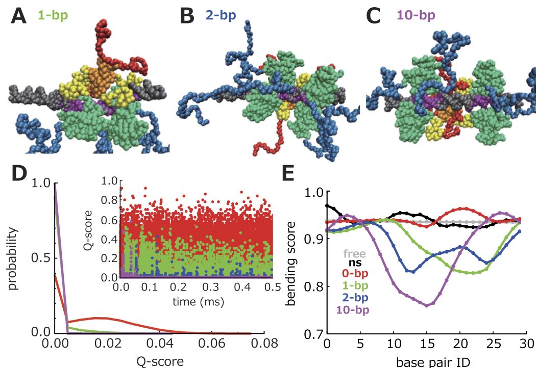
Figure 2. The p53-RE complex with varying spacer lengths. (A–C) Representative structures of the p53-RE complex in which the REs contain 1- (A), 2- (B), and 10- (C) bps spacers. (D) Probability distributions and time trajectories (inset) of Q-score of the inter-Core contacts of longitudinally aligned two Cores in which the RE contains 0- (red), 1- (green), 2- (blue), and 10-bps (magenta) spacers. (E) DNA bending scores vs base-pair IDs. The color assignment is the same as that of (D). We also plotted the scores of naked dsDNA (grey) and dsDNA to which p53 non-specifically binds (black).
