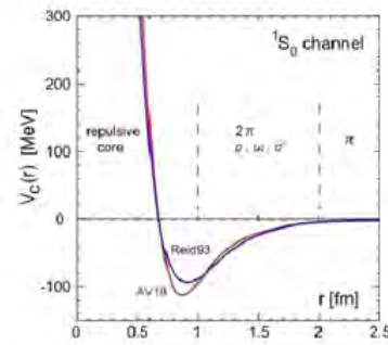
象論的核力ポテンシャルの例 Examples of phenomenological nuclear potential
