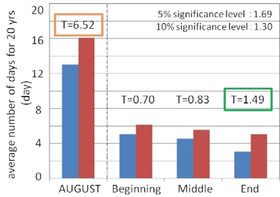
Fig. 8 The future change in the number of unsteady atmosphere events in August
