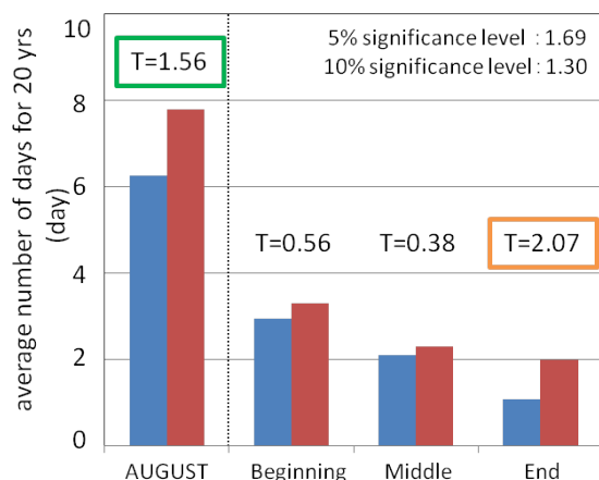
Fig.6 The future change in the number of events guerrilla-heavy rainfall in August
