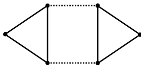
Figure 2. The graphical expression of the integral in (3.33) with possible derivatives on the solid lines.
