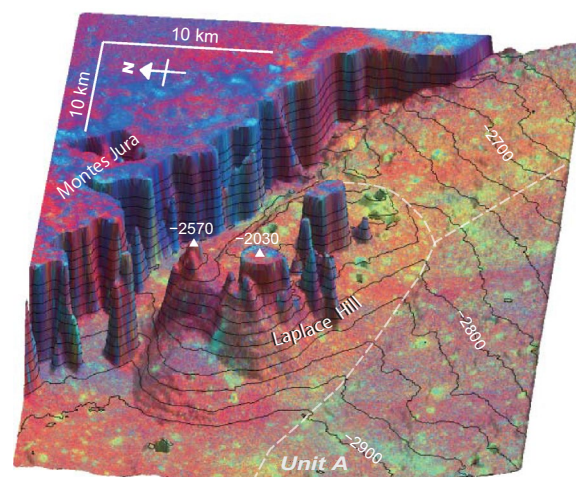
Fig. 16 Three-dimensional topographic models on which spectral ratio images are mapped. Topography around Laplace Hill. Montes Jura and peaks on the hill are truncated at -2600 m. Vertical exaggeration is 25. Contour interval is 25 m. Unit boundary is shown by a dashed line, a part of which lies along the southern foot of the hill. Triangle indicates a peak at the altitude of -2570 m
