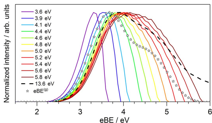
Fig. 3. eBE spectra of e_{aq}^- . eBE spectra for 12 different ionization laser energies 3.6 \text{ eV} \leq h\nu \leq 13.6 \text{ eV} (lines). The stars represent the genuine eBE (g) spectrum; that is, the spectrum devoid of scattering contributions. The genuine VBE (g) is 3.7 \pm 0.1 \text{ eV} . For clarity, only the calculated data from Fig. 2 are shown here. See fig. S9 for a comparison with the experiment.
