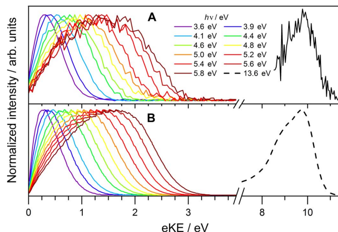
Fig. 2. Experimental and simulated photoelectron spectra of e_{aq}^- . Photoelectron kinetic energy distributions for 12 different ionization laser energies 3.6 \text{ eV} \leq h\nu \leq 13.6 \text{ eV} . All spectra are normalized to the same maximum intensity. (A) Experimental spectra. (B) Scattering simulations (section S2 and fig. S5).
