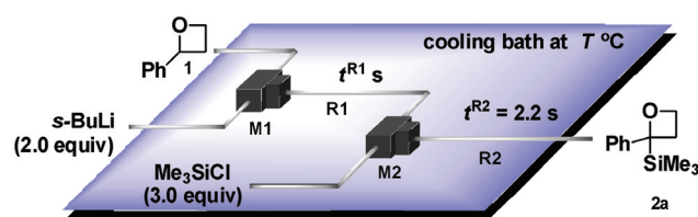
Figure 1: A flow microreactor system for the deprotonation of 2-Phenyloxetane ( 1 ) with s -BuLi followed by reaction with chlorotrimethylsilane. M1, M2: T-shaped micromixer. R1, R2: microtube reactor.
