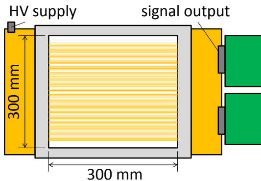
Figure 3. Outline of the wire chamber for BHCV.
