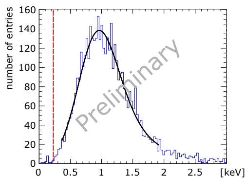
Figure 5. Energy deposit in a single wire chamber. The red dashed line shows a quarter of the peak used as threshold for efficiency calculation.
