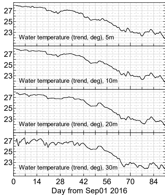
Fig.8 Temporal variations of water temperature from September to November
