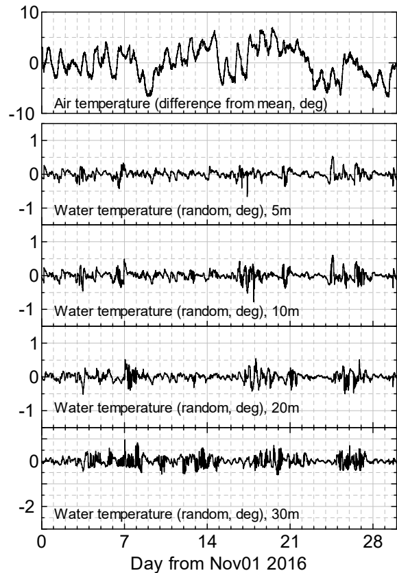
Fig. 10 Temporal variations of Air temperature (Top) and water temperature in November
