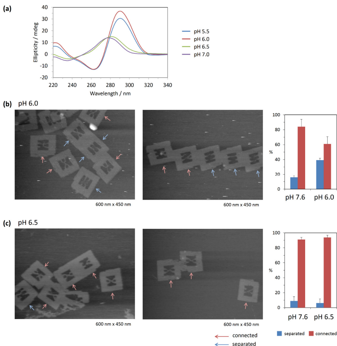
Figure S6. Separation of the GQ/i-motif duplex under the pH 6.0 and 6.5 conditions. (a) CD spectra of the i-motif forming sequence at pH 5.5, 6.0, 6.5, and 7.0. CD spectra were obtained in a solution containing 5 \mu M DNA strand, 10 mM MES buffer, 12.5 mM MgCl_2 . (b) AFM images of the DNA frame incubated at pH 6.0, which was prepared using the method shown in Figure 3. Summary of the proportions of GQ/i-motif duplex (connected) and separated strands at pH 7.6 (initial state) and pH 6.0. Blue and red arrows in the AFM images indicate the separated and connected (X-shaped) strands, respectively. (c) AFM images of the DNA frame incubated at pH 6.5. Summary of the proportions of GQ/i-motif duplex (connected) and separated strands at pH 7.6 (initial state) and pH 6.5.
