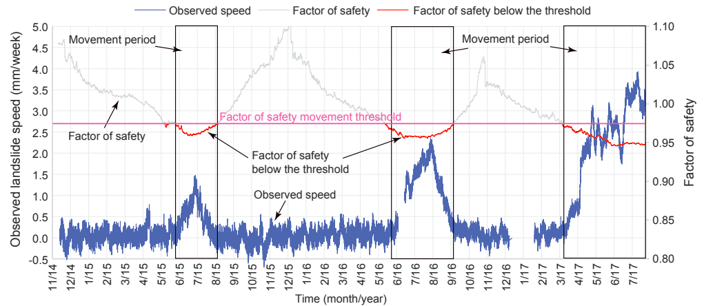
Figure 3. Results from landslide stability modeling considering resistance from variable swell pressure. Factor of safety ( F ) was calculated using measured parameters and equation (3). The approximate threshold factor of safety was selected to capture all movement periods, and F is emphasized (with red color) when it is below the threshold; this threshold predicts movement that strongly correlates with observed movement.
