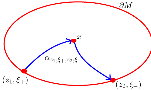
FIGURE 3. Broken geodesic data consists of initial direction (z_1, \xi_+) , final direction (z_2, \xi_-) and total length of broken geodesic \alpha_{z_1, \xi_+, z_2, \xi_-} .
