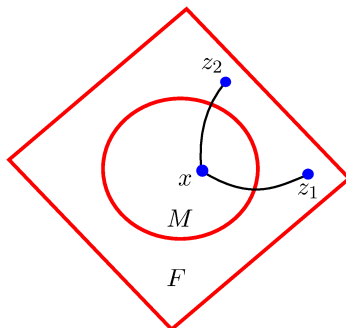
FIGURE 2. Distance difference function D_x(z_1, z_2) = d(x, z_1) - d(x, z_2) of the point x \in M is evaluated at the points z_1, z_2 \in F = \overline{U} \setminus M . Note that below we will assume for simplicity that the boundaries of M and U are smooth.
