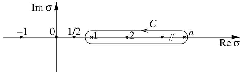
Figure 3. Contour of integration for (35). ( x : poles of the integrand.)
