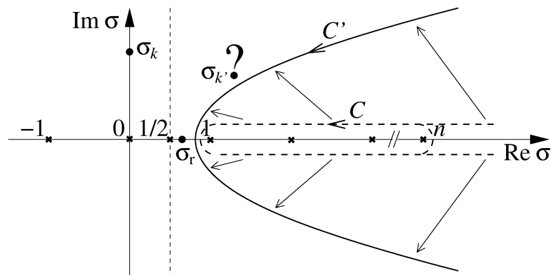
Figure 4. Integration-path deformation for a large- n evaluation of the integral (35). • : typical saddle-points (none on scale); \sigma_k(n) comes from a Riemann zero \frac{1}{2} + i\tau_k on the critical line (and is irrelevant, beyond reach), \sigma_{k'}(n) comes from a putative (“?”) zero \frac{1}{2} + i\tau_{k'} off the critical line (and then, gives a dominant contribution), finally \sigma_r(n) is the real saddle-point tending to the pole \sigma = 1/2 from above (and gives the dominant contribution if and only if RH holds).
