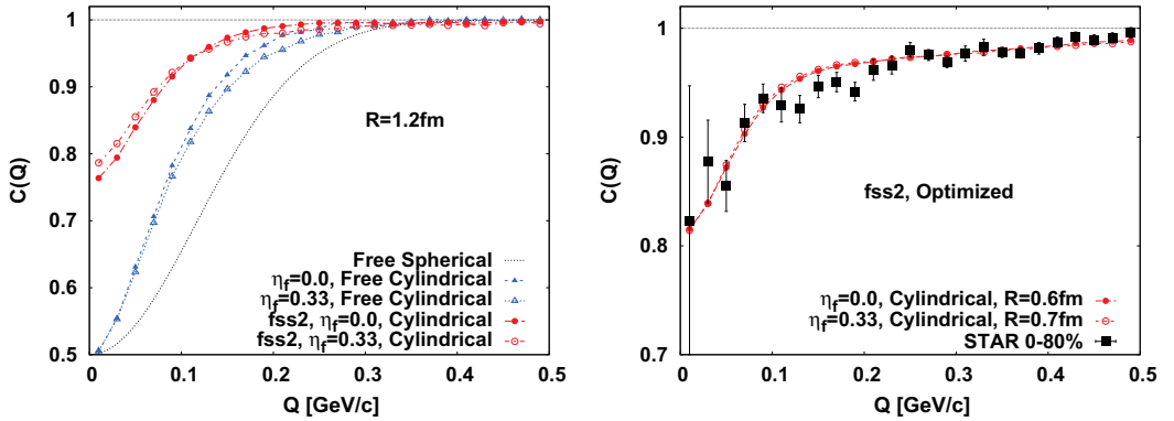
Figure 2. \Lambda\Lambda correlation function for R = 1.2 fm. Left: Comparison of the free cases and interacting cases with and without flow. Right: R is optimized for the STAR data.
