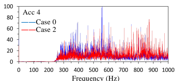
Fig. 20 Transfer function in the vertical motion for Case 0 and Case 2 by Rinkai wave input
