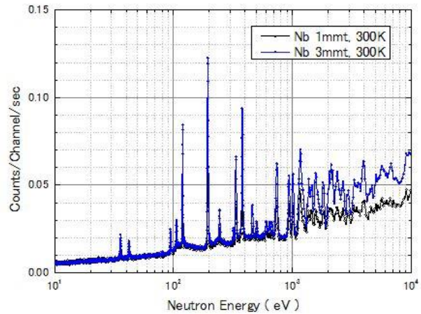
Fig1. Measured TOF spectrum
