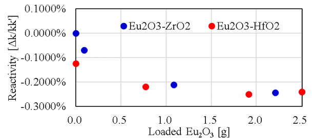
Fig. 3 Reactivity Measurement Results of Eu 2 O 3 -ZrO 2 or Eu 2 O 3 -HfO 2 .
