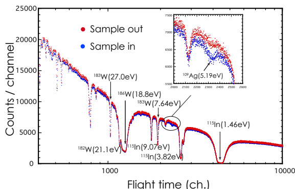
Fig. 1. TOF spectrum with pulse width 0.1 \mu s
