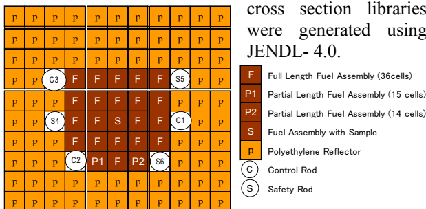
Fig. 1 Configuration of E3 core assembled in KUCA A-core.
