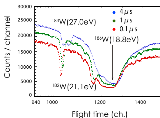
Fig. 2. The TOF spectra of individual pulse widths
