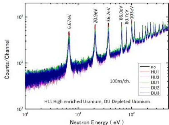
Fig.1 Comparison of TOF spectra with and without samples
