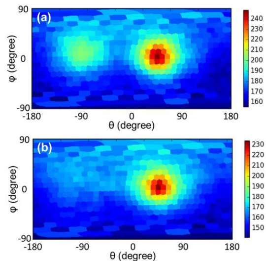
Fig. 3. Reconstructed images on the projection sphere ( \theta , \varphi ), (a) with the ^{10}\text{B} sample and (b) with a dummy sample not including ^{10}\text{B} .
