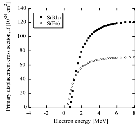
Fig. 1 Primary displacement cross section as a function of electron energy.
