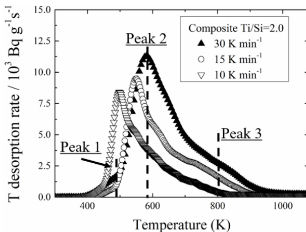
Fig. 2. Tritium-TDS spectra of composite Ti/Si=2.0 at different heating rates.
