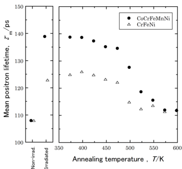
Fig. 1 Mean positron lifetime in the electron-irradiated CoCrFeMnNi and CrFeNi alloys after isochronal annealing.
