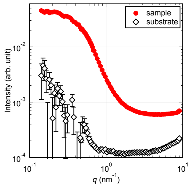
Fig. 1. SAXS profiles of a semiconductor nanocomposite thin film and a Si substrate.
