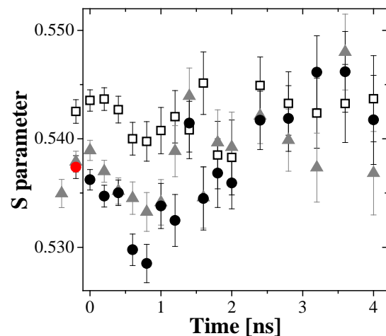
Fig. 2. Line-shape parameter S as a function of time (positron age) for gamma-ray irradiated polystyrene at various doses: \square un-irradiated, \blacktriangle 30-kGy, and \bullet 300-kGy.
