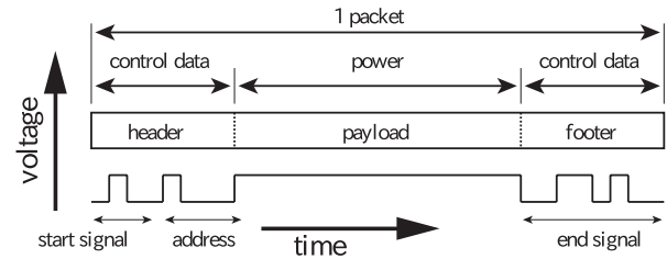
Fig. 2 Configuration of a power packet.
