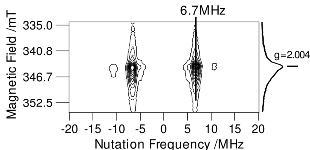
FIG. 2. 2D-ESTN spectrum of BaTiO 3 observed at 10 K. The nutation pulse- \pi/2 (16 ns)- \tau - \pi (32 ns)- \tau -echo detection sequence was applied.
