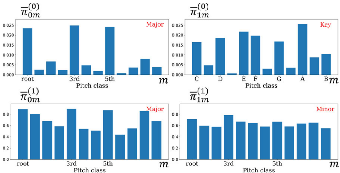
Fig. 6. The emission probabilities \bar{\pi} obtained by the tatum-level model assuming the sequential dependency of \mathbf{S} .
