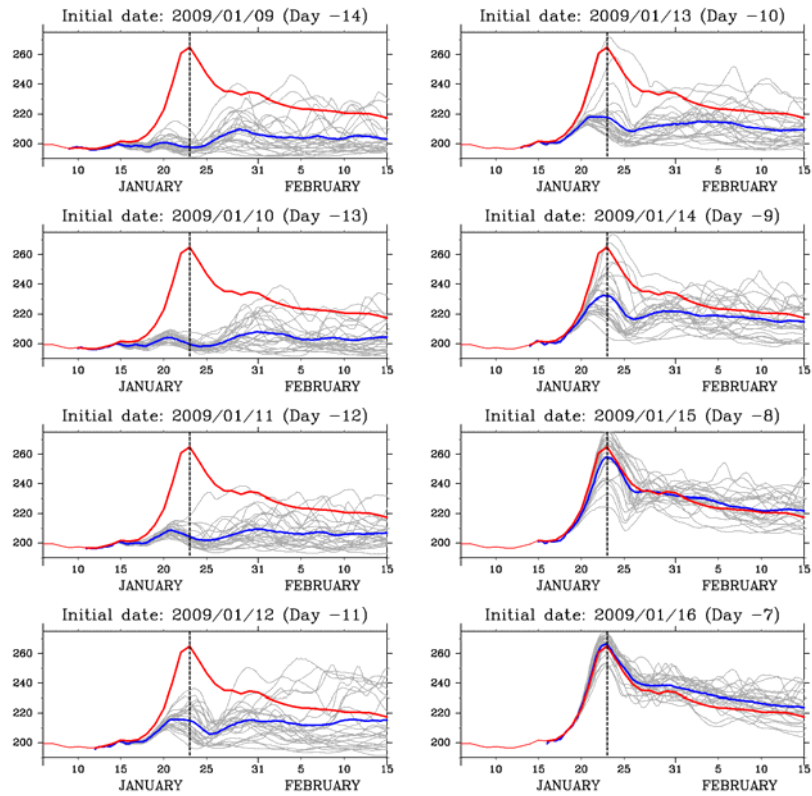
Fig. 3 Prediction of 10 hPa temperature (unit; K) averaged poleward of 80°N during the 2009 SSW event. The red line indicates the analysis, the black line the prediction of each ensemble member, and the blue line the corresponding ensemble mean prediction.
