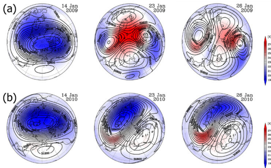
Fig. 2 Horizontal distribution of geopotential height (contour; unit: m) and temperature (color shade, unit: K) at 10 hPa during the 2009 SSW event (a) and the 2010 SSW event (b).
