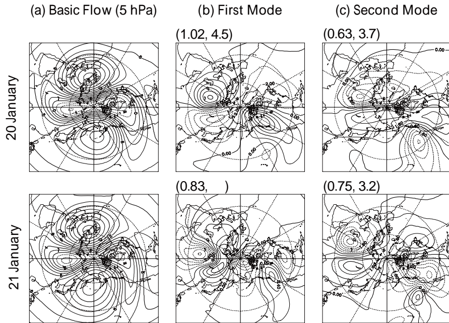
Fig. 8 (a) Horizontal structure of the basic flow given by the T21 truncated 5-hPa streamfunction field ( 10^7 \text{ m}^2 \text{ s}^{-1} ) of day-4 ensemble mean prediction. (b) and (c) show streamfunction field of the first and second unstable modes computed for the basic flow shown in panel (a). The first and second numbers in parentheses above each panel indicate the growth rate ( \text{day}^{-1} ) and the period (days) of the unstable mode, respectively. A Stationary mode with zero imaginary component of the eigenvalue is designated by the period of the infinity. Upper (lower) panels are for 20 January (21 January) 2009.
