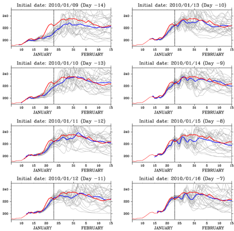
Fig. 4 As in Fig.3, except for the 2010 SSW event.
