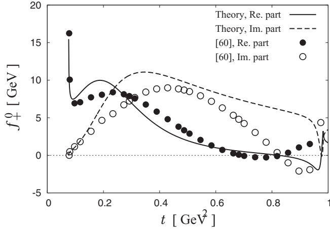
FIG. 11. Frazer–Fulco amplitude f_+^0 for the N\bar{N} \rightarrow \pi\pi reaction. Points represent quasi-empirical values taken from Ref. [60].
