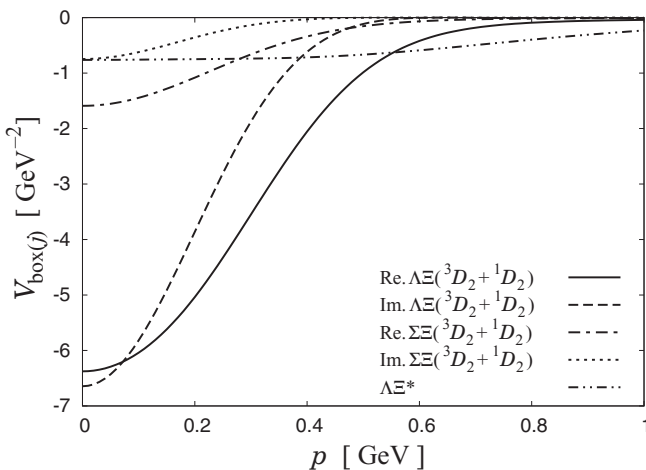
FIG. 6. The inelastic contributions to the N\Omega(^5S_2) interaction V_{\text{box}(j)}(E; p, p) as functions of momentum p . The energy in the effective interaction is fixed as E = m_N + m_\Omega . In the figure \Lambda\Xi and \Sigma\Xi indicates the sum of ^3D_2 and ^1D_2 contributions, respectively.
