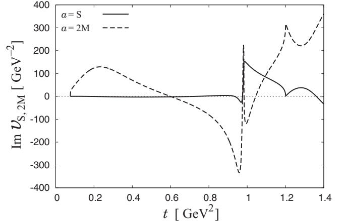
FIG. 13. \text{Im}\mathcal{V}_S and \text{Im}\mathcal{V}_{2M} in our model.
