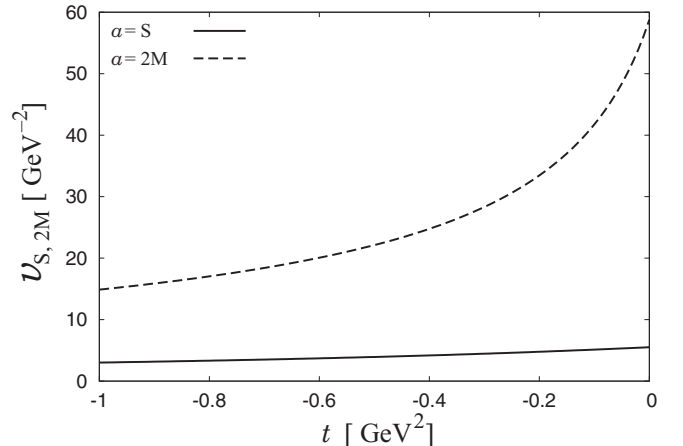
FIG. 3. Lorentz invariant amplitudes \mathcal{V}_S and \mathcal{V}_{2M} calculated with the dispersion relation as functions of the Mandelstam variable t .
