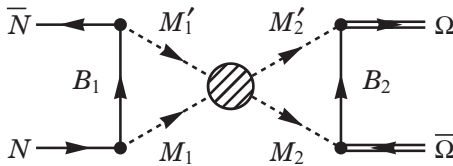
FIG. 2. Feynman diagram for the N\bar{N} \rightarrow \Omega\bar{\Omega} reaction. Particles in the intermediate states are listed in Table II. Shaded circle denotes the correlation of two mesons.
