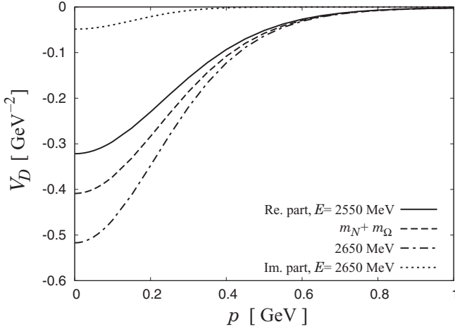
FIG. 5. The D -wave contribution to the N\Omega(^5S_2) interaction V_D(E; p, p) as a function of momentum p . The energy in the effective interaction is fixed as E = m_N + m_\Omega , 2550 MeV, and 2650 MeV. Because the energy is above the N\Omega threshold, the contribution at E = 2650 MeV has an imaginary part.
