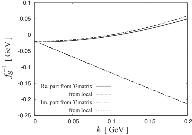
FIG. 7. Inverse of scattering amplitude f_S^{-1} . In addition to f_S^{-1} calculated from the T matrix, we also plot f_S^{-1} from the equivalent local N\Omega potential (see Sec. V). We note that the two lines of the imaginary parts almost overlap each other.
