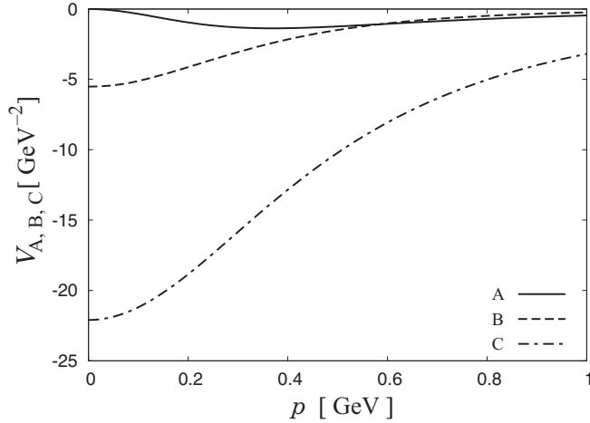
FIG. 4. The elastic contributions to the N\Omega(^5S_2) interactions V_A(p, p) , V_B(p, p) , V_C(p, p) as functions of momentum p .
