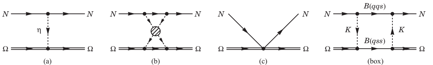
FIG. 1. Feynman diagrams for the N\Omega interaction. The dashed lines represent the pseudoscalar mesons, while the solid and double lines indicate baryons. Shaded circle denotes the correlation of two mesons, and B(qqs)B(qss) represents \Lambda \Xi , \Sigma \Xi , and \Lambda \Xi(1530) .
