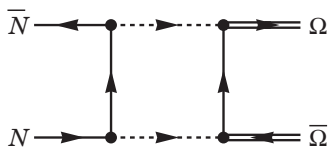
FIG. 12. Feynman box diagram for the N\bar{N} \rightarrow \Omega\bar{\Omega} reaction. Solid and double lines in the intermediate state represent baryons, and dashed lines represent mesons.
