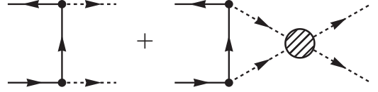
FIG. 10. Diagrammatic equation for the N\bar{N} \rightarrow P\bar{P} and \Omega\bar{\Omega} \rightarrow P\bar{P} scattering amplitudes. Solid and dashed lines represent baryons and mesons, respectively. Shaded circle denotes the correlation of two mesons.
