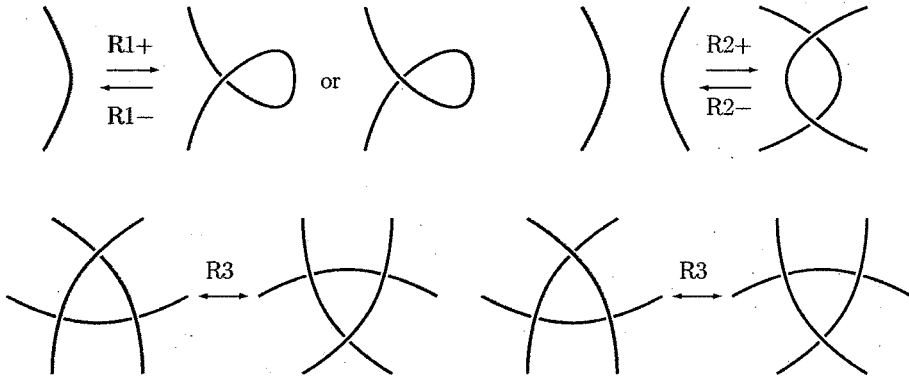
FIGURE 1. Reidemeister moves
