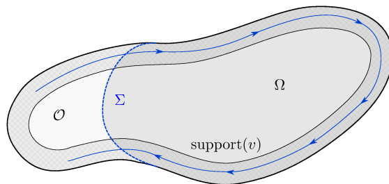
Figure 4: The kaitenzushi strategy
