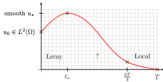
⊠ 2: Reduction to a global approximate controllability problem
