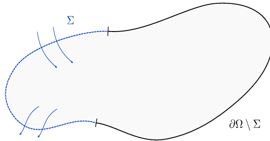
⊠ 1: The control problem
