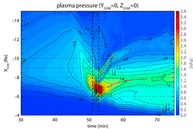
Figure 1. Temporal variation of simulated plasma pressure as a function of X_{GSM} in the equatorial plane ( Y_{GSM} = 0 and Z_{GSM} = 0 Re). The vertical dashed lines refer to the time at elapsed times of 51 and 52.8 min. The horizontal lines give reference from X_{GSM} = -6 to -10 Re with 1 Re interval. The red thick curve and line indicate evolution of the main part and sub part of the high-pressure region after the substorm onset, respectively.
