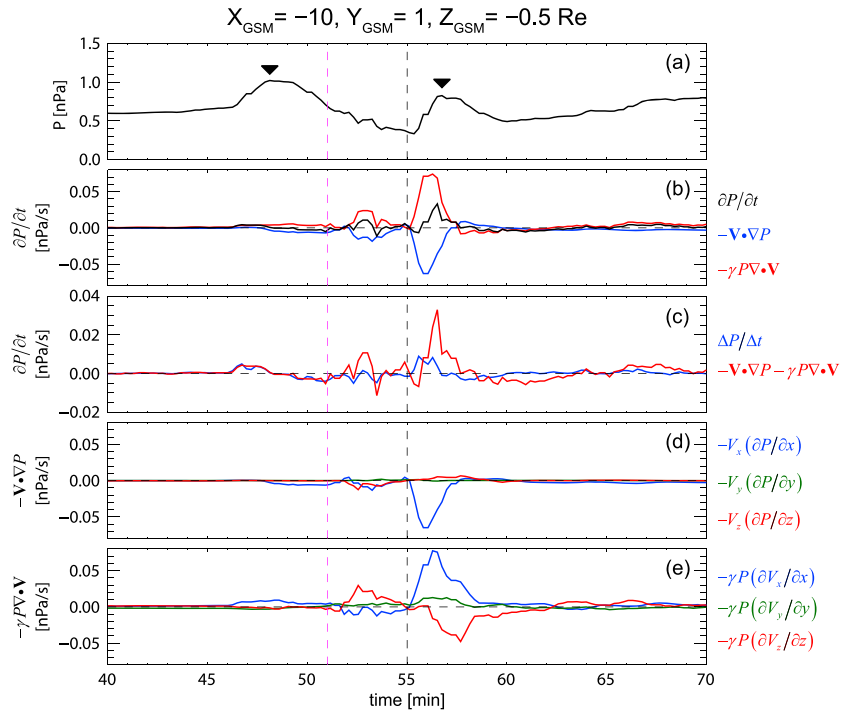
Figure 6. Temporal variation of simulated (a) plasma pressure, (b) \partial P/\partial t , term 1 ( -Vg\nabla P ) and term 2 ( -\gamma P\nabla gV ) on the right-hand side of the equation (5) in the black, blue, and red lines, respectively, (c) \partial P/\partial t in blue line, and ( -Vg\nabla P - \gamma P\nabla gV ) in red line, (d) three subterms of the term 1, (e) three subterms of term 2. The two vertical dashed lines indicate the time at 51 and 55 min.
