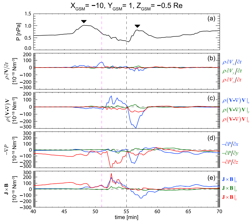
Figure 5. Temporal variation of simulated force terms defined in the equation (4) at coincident position of probe THE in the MHD frame. (a) Plasma pressure, (b) \rho(\partial V/\partial t) , (c) \rho(\mathbf{V}\cdot\nabla)\mathbf{V} , (d) plasma pressure gradient force, and (e) Lorentz force. The two vertical dashed lines indicate the time at 51 and 55 min.
