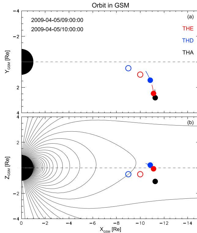
Figure 2. Orbit of THEMIS probes (THD, THE, and THA) shown by solid circle (start point) with line pointing the orbit in (a) X_{GSM} - Y_{GSM} and (b) X_{GSM} - Z_{GSM} planes during the period between 09:00 and 10:00 UT on 5 April 2009. The open circles refer to coincident positions of the associated THEMIS probes in the MHD simulation domain (see text for details).
