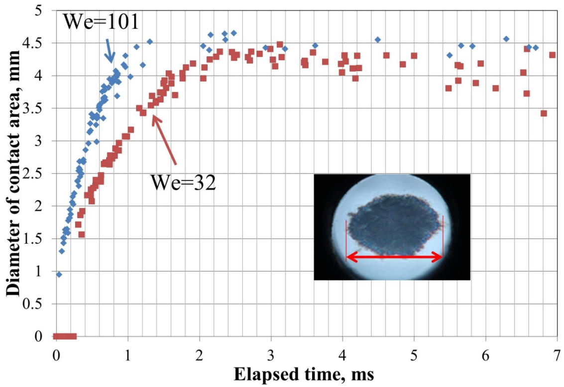
Fig.9 Time evolution of contact diameters for We=101 and 32 at 500\text{ }^{\circ}\text{C}
