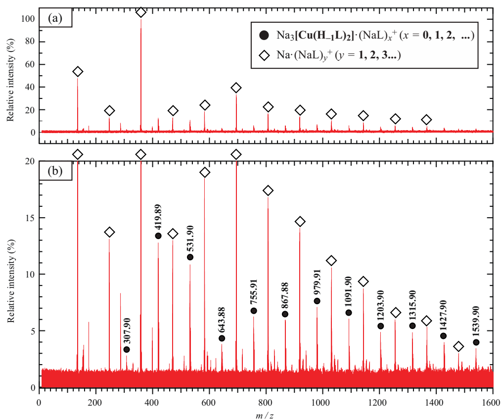
Figure 4. (a) Full and (b) enlarged PESI-MS spectra of an aqueous solution of 0.4 M copper(II)–3.0 M lactate at c_{NaOH} = 3.7 M, acquired without sample dilution.
