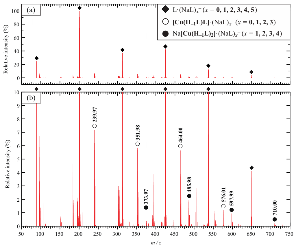
Figure 3. (a) Full and (b) enlarged ESI-MS spectra of a 1000-fold-diluted supernatant aqueous solution of 0.4 M copper(II)–3.0 M lactate at c_{NaOH} = 3.7 M.
