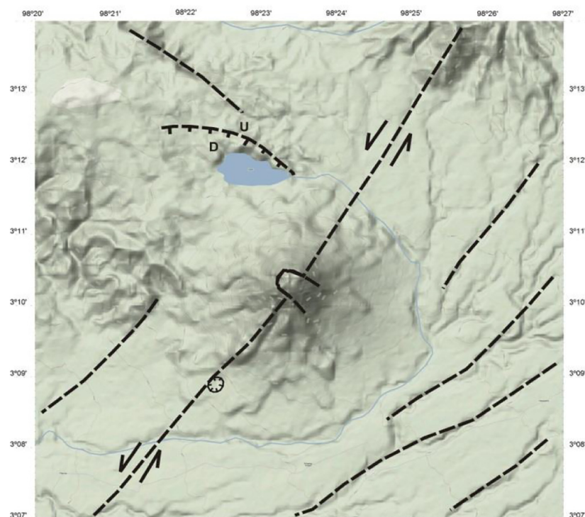
Fig. 7. Geological map of Sinabung volcano (Prambada, 2010). Black dashed line with arrow is strike slip fault across the Sinabung volcano.
