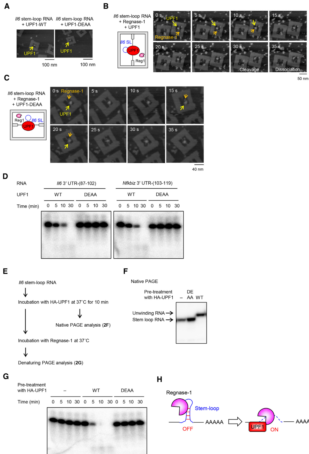
Figure 2. The unwinding of stem-loop by RNA helicase UPF1 induces RNA cleavage by Regnase-1. (A) AFM images of complex of DNA frame with //6 RNA and UPF1. (B and C) Time-lapse AFM images of complex of DNA frame with indicated //6 stem-loop RNA, Regnase-1 and UPF1. Time 0 s is an arbitrary time during the AFM scanning. Scanning rate is 0.2 frames/s. (D) Regnase-1 cleaved the stem-loop RNAs in the presence of UPF1 in vitro . Indicated 5'- 32 P-labeled RNAs were incubated with Regnase-1 and HA-UPF1 for indicated time, and analyzed by TBE-urea gel electrophoresis. (E) Flow chart depicting experiments where 5'- 32 P-labeled //6 stem-loop RNA was incubated with UPF1 at 37°C for 10 min, purified at 4°C and analyzed by native PAGE electrophoresis. To keep unwinding structure of stem-loop RNA by UPF1, RNA was immediately incubated and kept at 4°C after UPF1 treatment, and then incubated with Regnase-1. (F) Native PAGE analysis of //6 stem-loop RNA treated with UPF1. (G) Regnase-1 cleaved the //6 stem-loop RNA treated with UPF1 in vitro . The //6 stem-loop RNA treated with UPF1 were incubated with Regnase-1 for indicated time and analyzed by TBE-urea gel electrophoresis. (H) Schematic illustration showing that the unwinding of stem-loop by UPF1 induces RNA cleavage by Regnase-1. See also Supplementary Figure S1 and Supplementary Movies S3 and S4.
