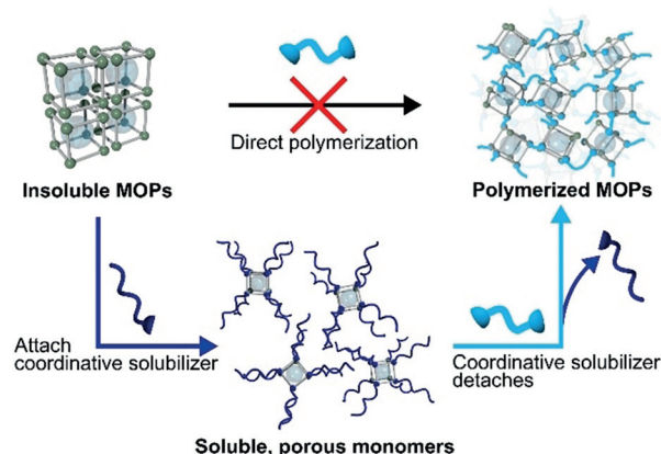
Figure 1. The strategy used in this paper to solubilize MOPs. Assemblies of insoluble MOPs are made soluble by the attachment of a monodentate, coordinative solubilizer. These monodentate ligands can then be replaced with bidentate linkers, driving the assembly of the MOPs into porous polymers.
