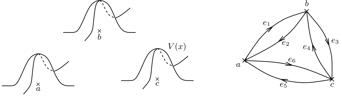
Figure 1. Three bumps potential and the graph of trapped set
