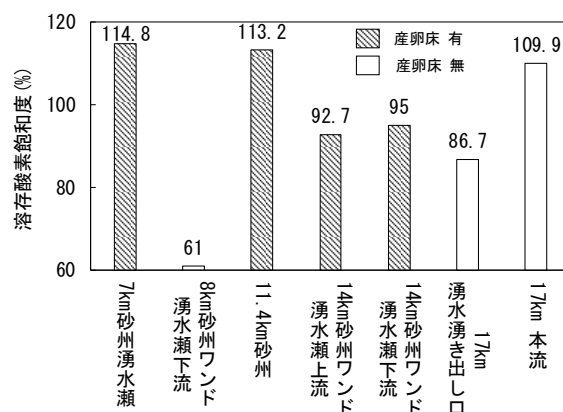
Fig. 9 Dissolved Oxygen at survey sites in the spring channels in the Tenryu River.
