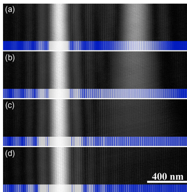
Fig. 4. Series of the experimental results by changing the right slit width w_{\text{right}} : (a) w_{\text{right}} = 38 nm, (b) 22 nm, (c) 10 nm and (d) 5 nm. The defocus distance \Delta f was 23.2 mm for all panels. Inset images in blue at the bottom of each panel are calculated results along the yellow lines in Fig. 2.
