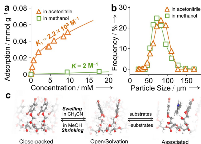
Figure 1. (a) Adsorption isotherms using diphenylurea as a substrate and poly1 as a stationary phase in acetonitrile (triangle) and methanol (square) at 293 K. The former gave a bi-Langmuir plot with K_1 = 2.2 \times 10^3 \text{ M}^{-1} and K_2 = 25 \text{ M}^{-1} . For details, see Figure S3 in the Supporting Information. (b) DLS plot of poly1 in acetonitrile (triangle) and methanol (square) at 293 K ( n=3 ). (c) The reaction scheme for the association between poly1 and substrates. White: hydrogen; gray: carbon; blue: nitrogen; red: oxygen; brown: bromine. The solvent was omitted for clarity.
