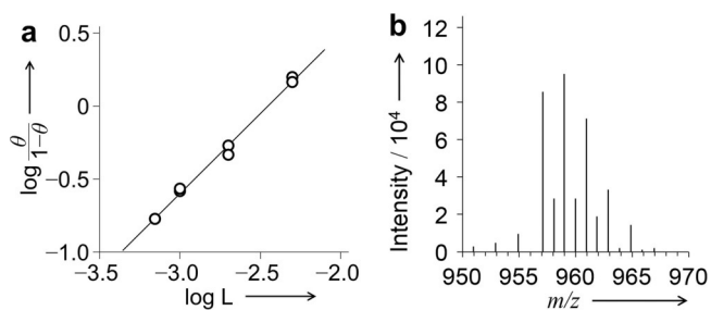
Figure 3. (a) A modified Hill plot for the 1 + diphenylurea pair in acetonitrile at 283 K showing the relationship between \log[\theta/(1-\theta)] and the logarithm of the substrate concentration. For the derivation of the equations, see the Supporting Information. (b) Mass spectrum of the 1 + diphenylurea pair with a negative mode.
