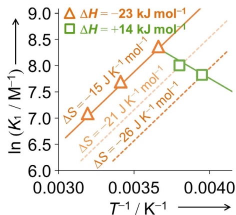
Figure 4. Arrhenius-type plot of \ln K_1 using poly 1 as the stationary phase and diphenylurea as the substrate in acetonitrile. The \ln K_1 values were determined by using a constant \theta_{\text{sat}} of 27 \mu\text{mol g}^{-1} . The original data are shown in Figure S3 and Table S1 of the Supporting Information.
