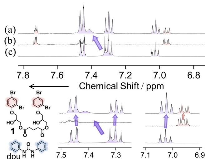
Figure 2. 1 H NMR spectra of (a) 1 + diphenylurea, (b) 1, and (c) diphenylurea in [D 3 ]acetonitrile at 293 K.
