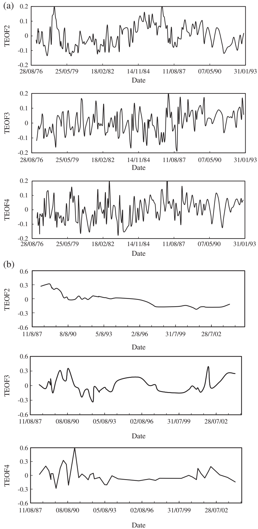
Fig. 8. a. Temporal EOFs of Narrabeen Beach profiles at Profile 4. b. Temporal EOFs of Milford-on-Sea Beach profiles at Profile 5F00107. c. Temporal EOFs of Hasaki Coast profiles at Hazaki Pier. d. Temporal EOFs of Joetsu-Ogata Coast profile.
