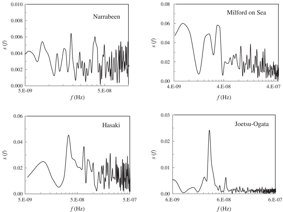
Fig. 9. Spectra of incident wave heights at four study sites.
