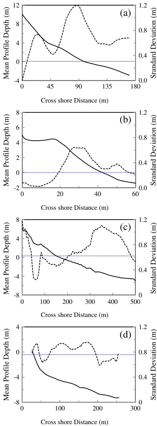
Fig. 5. Time mean beach profiles and standard deviation. (a) Narrabeen Beach, (b) Milford-on-Sea Beach, (c) Hasaki Coast, and (d) Joetsu-Ogata Coast. Blue dotted line shows the mean water level.
