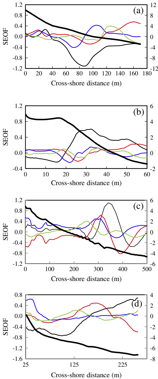
Fig. 7. First five spatial eigenfunctions of beach profiles at four study sites. (a) Narrabeen Beach; (b) Milford-on-Sea beach; (c) Hasaki coast; and (d) Joetsu-Ogata coast. Primary axis corresponds to SEOF2 to SEOF5. Secondary axis corresponds to SEOF1. Dark black line resembles mean profile. Black line SEOF2, red line SEOF3, blue line SEOF4 and green line SEOF5.
