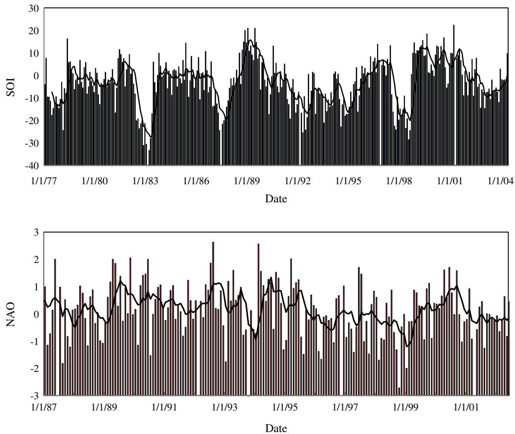
Fig. 10. (a) ENSO driven monthly Southern Oscillation Index during 1977 and 2004 ( http://www.bom.gov.au/climate/current/soihtm1.shtml ) (top). North Atlantic Oscillation ( http://www.cpc.ncep.noaa.gov/products/precip/CWlink/pna/nao_index.html ) (bottom). (Black line– 6 monthly moving average).
