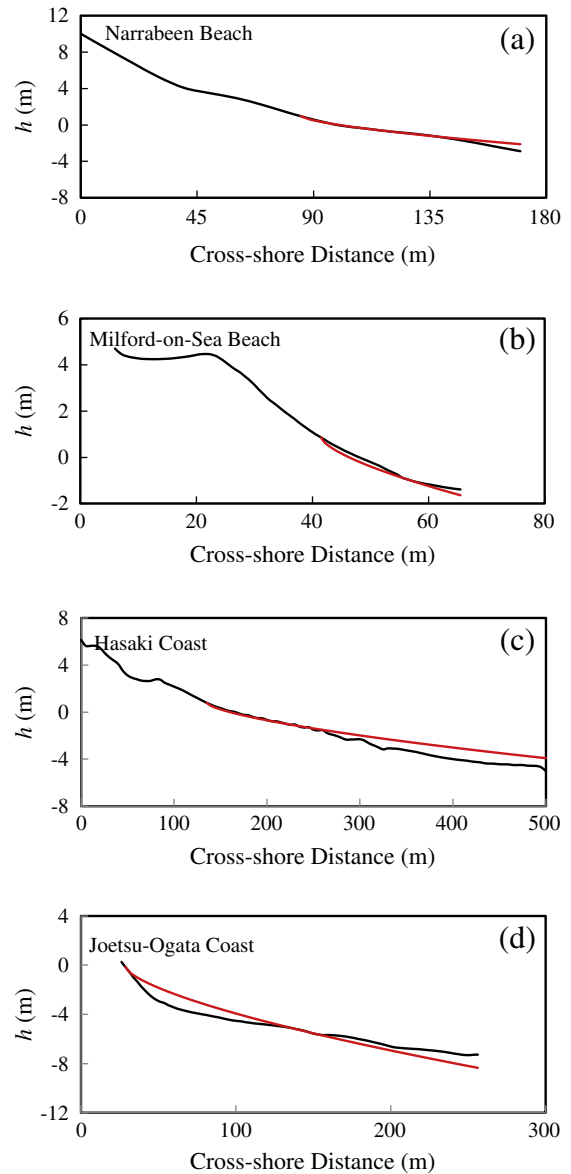
Fig. 6. Comparison of measured mean beach profile and Dean's Equilibrium profile. (a) Narrabeen Beach, (b) Milford-on-Sea Beach, (c) Hasaki Coast, and (d) J-O Coast. Black line – mean profile, red line – Dean's equilibrium profile.
