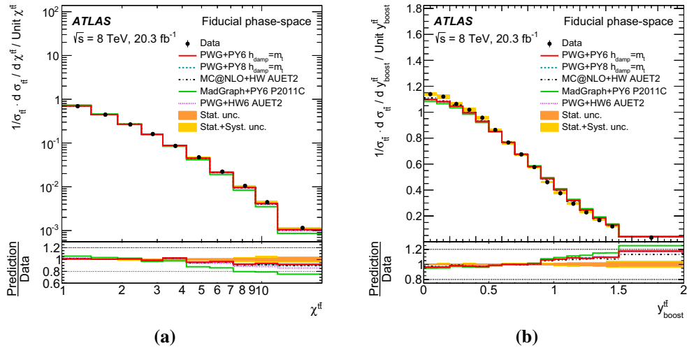
Fig. 7 Fiducial phase-space normalized differential cross-sections as a function of the t\bar{t} a production angle ( \chi^{t\bar{t}} ) and b longitudinal boost ( y_{\text{boost}}^{t\bar{t}} ). The yellow bands indicate the total uncertainty on the data in
