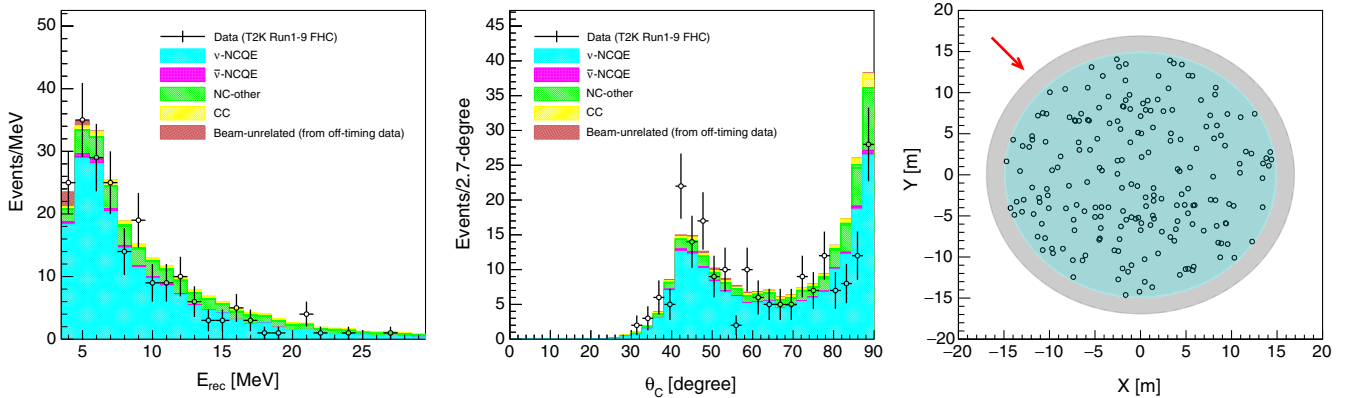
FIG. 7. Distributions of E_{\text{rec}} (left), \theta_C (middle), and vertex (right) from the FHC sample. In the right panel, the red arrow indicates the beam direction and the grey and sky blue regions correspond to the ID and FV, respectively.
