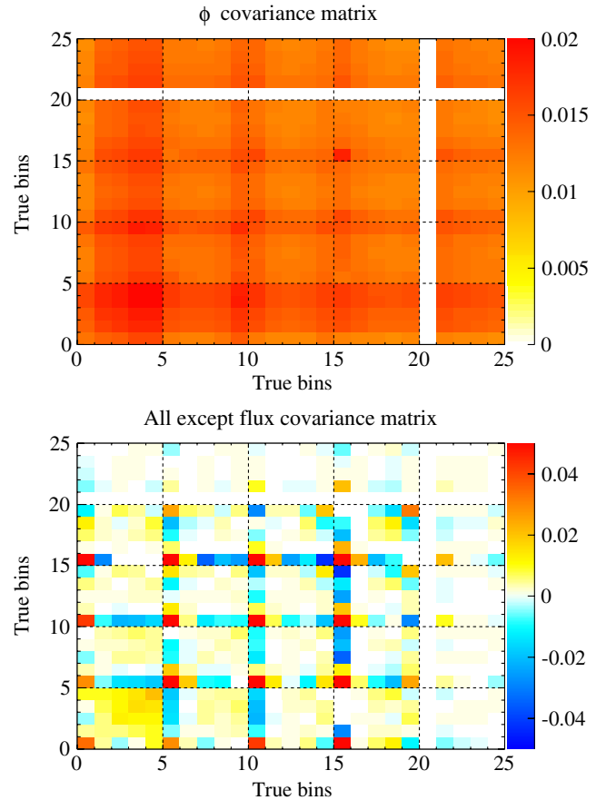
FIG. 11 (color online). The fractional covariance matrix obtained from the uncertainties on the flux (top), and uncertainties due to all sources except the flux (bottom). The x -axis and y -axis bin numbering is defined in Table XI.
