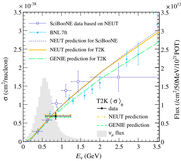
FIG. 13 (color online). The T2K total flux-averaged cross section with the NEUT and the GENIE prediction for T2K and SciBooNE. The T2K data point is placed at the flux mean energy. The vertical error represents the total (statistical and systematic) uncertainty, and the horizontal bars represent 68% of the flux at each side of the mean energy. The T2K flux distribution is shown in grey. The predictions for SciBooNE have been done for a \text{C}_8\text{H}_8 target [52] which is comparable to the mixed T2K target. BNL data has been measured on deuterium [53].
