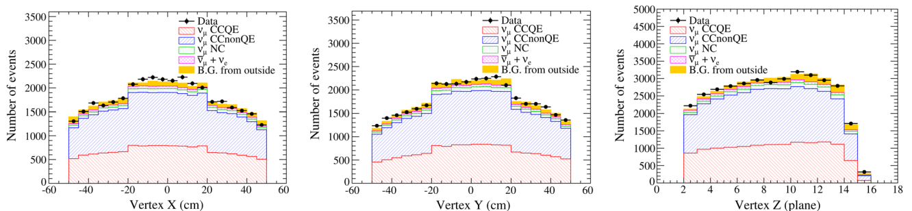
FIG. 10 (color online). Vertex X, Y, and Z distributions for the proton module following event selection. There are jumps at X or Y = \pm 20 cm because the proton module uses thicker scintillators in the inner region ( -20 cm \sim +20 cm).
