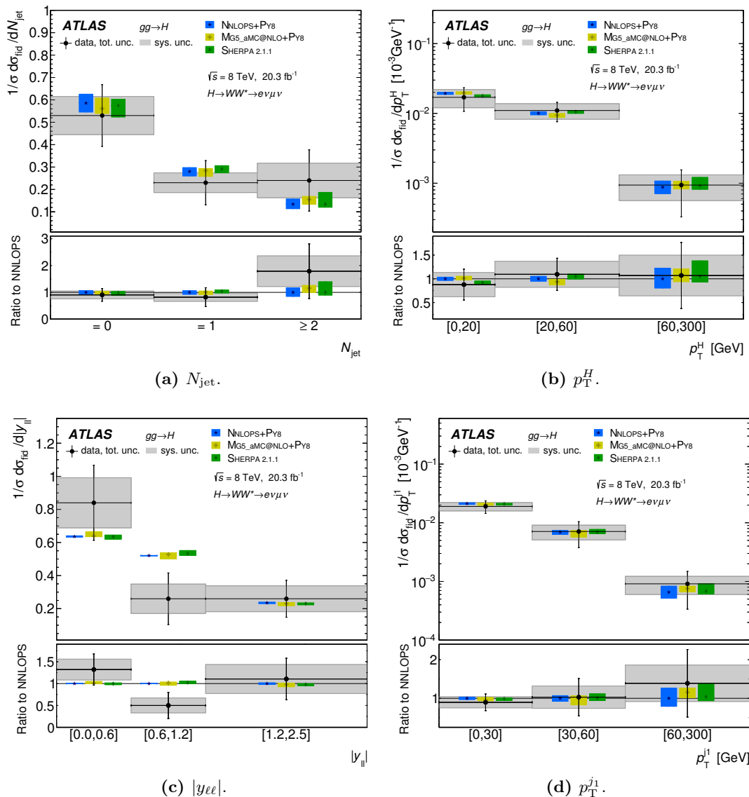
Figure 7. Normalised fiducial differential cross section measurements as a function of (a) N_{\text{jet}} , (b) p_T^H , (c) |y_{\ell\ell}| , and (d) p_T^{j_1} , overlaid with the signal predictions. The [0, 30] GeV bin of the p_T^{j_1} distribution includes events with no reconstructed jets. The systematic uncertainty at each point is shown by a grey band labelled “sys. unc.” and includes the experimental and theoretical uncertainties. The uncertainty bar, labelled “data, tot. unc.” is the total uncertainty and includes all systematic and statistical uncertainties. The measured results are compared to various theoretical predictions.
